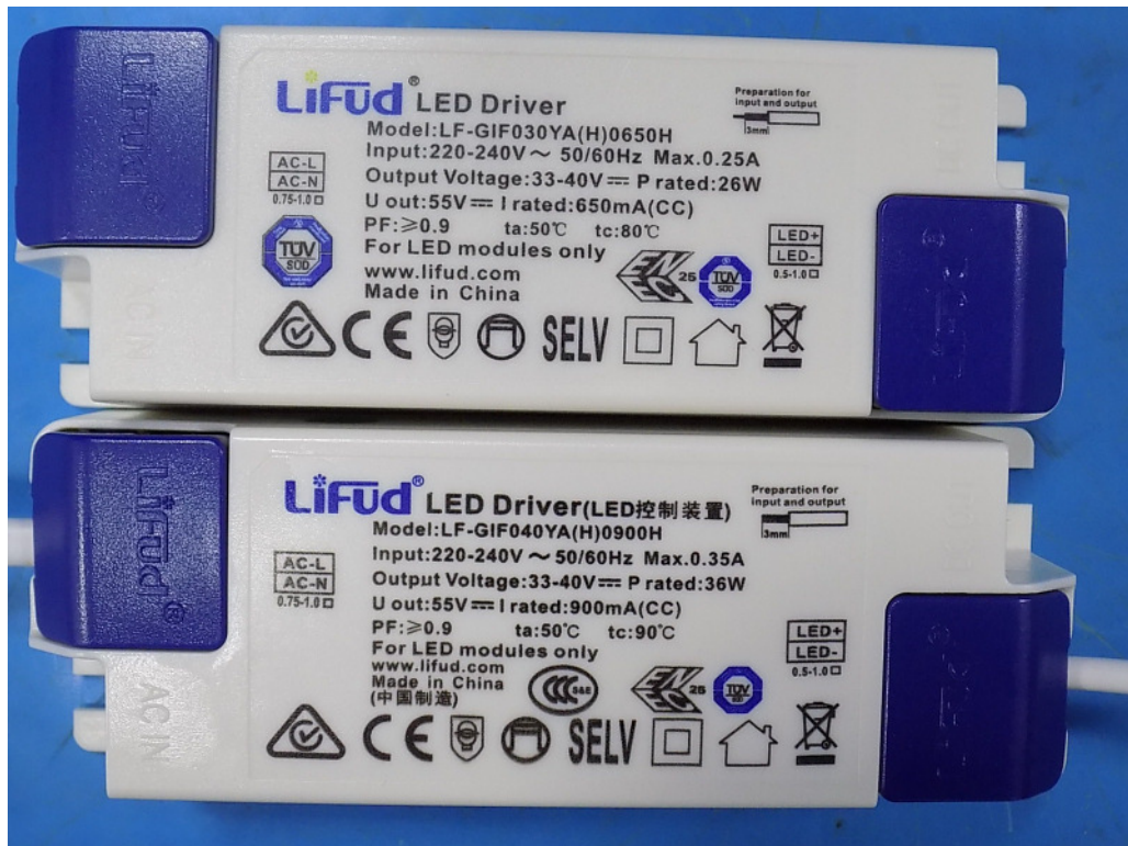
Figure 16: the front view of LF-GIF040YA(H)-xxxxxy / LF-GIF030YA(H)-xxxxxy
